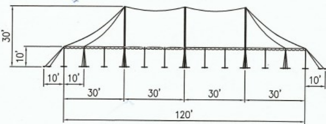
SIDE ELEVATION
